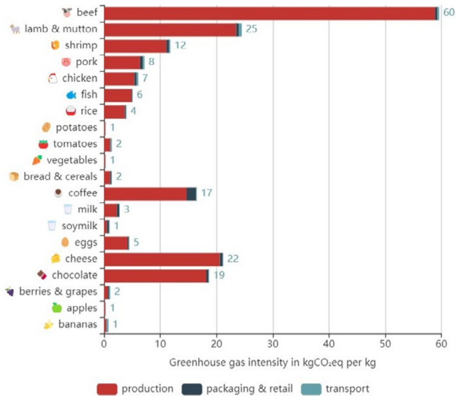
Figur 16. Nerisassat immikkut toqqakkat, taakkulu CO 2 -aftrykii. Tigulaariffik: https://ourworldindata.org/food-choice-vs-eating-local
