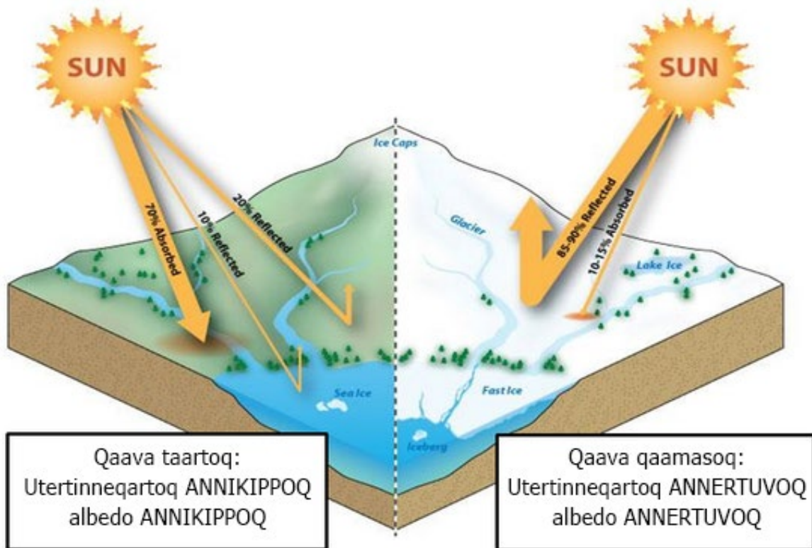
Ilusiliaq 10: Albedo. Aallerfik: DMI ( https://www.dmi.dk/nyheder/2019/forstaa-faenomenet-tipping-points/ ).
